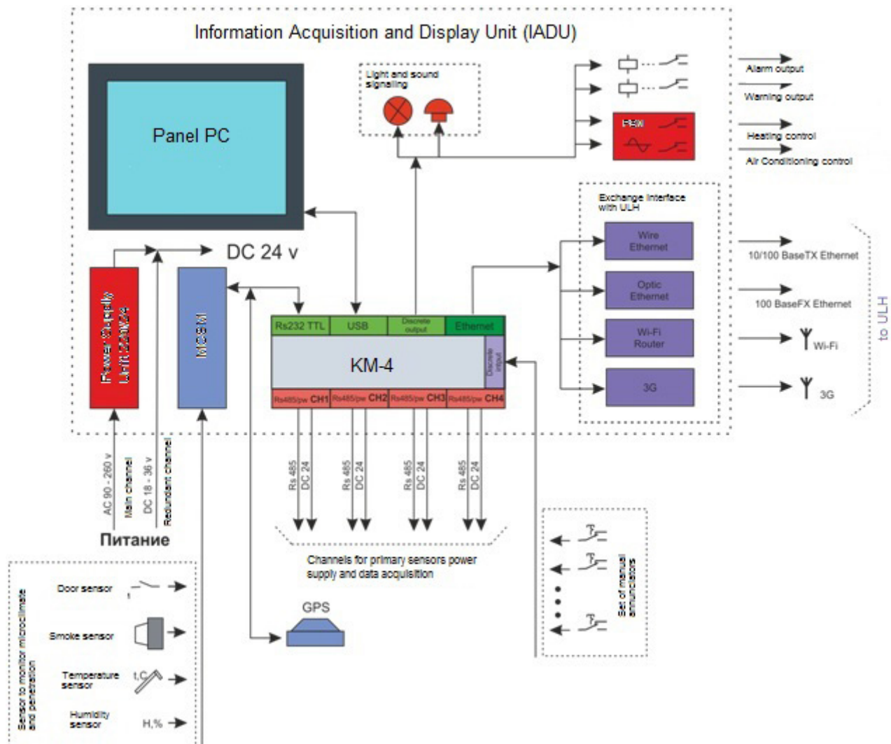
Fig.3 Block diagram of IADU and periphery interaction
